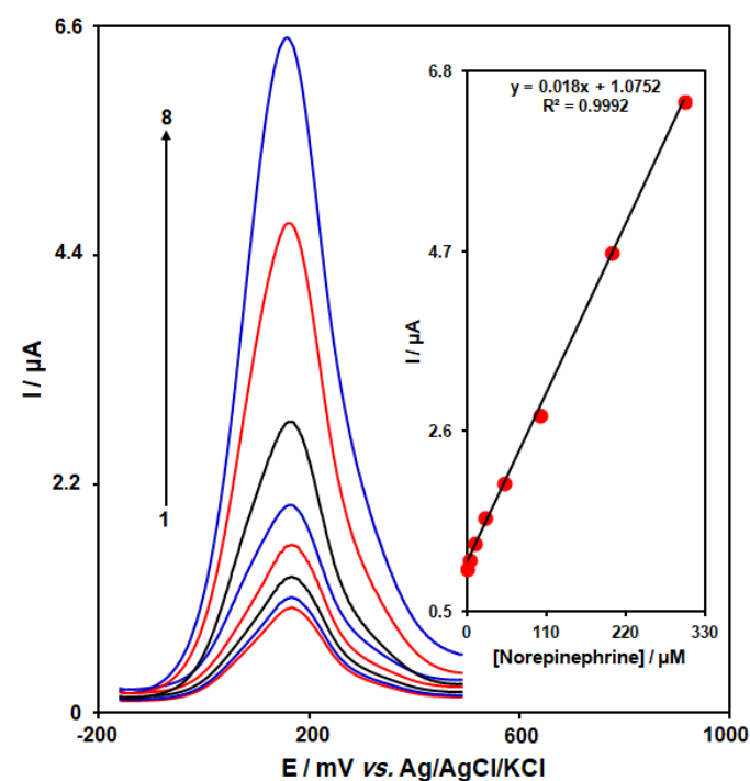
Fig. 5. DPVs of Cu/SPE in 0.1 M (pH 7.0) containing different concentrations of norepinephrine. Numbers 1–8 correspond to 0.3, 2.5, 10.0, 25.0, 50.0, 100.0, 200.0 and 300.0 \mu\text{M} of norepinephrine. Inset: plot of the electrocatalytic peak current as a function of norepinephrine concentration in the range of 0.3–300.0 \mu\text{M}
