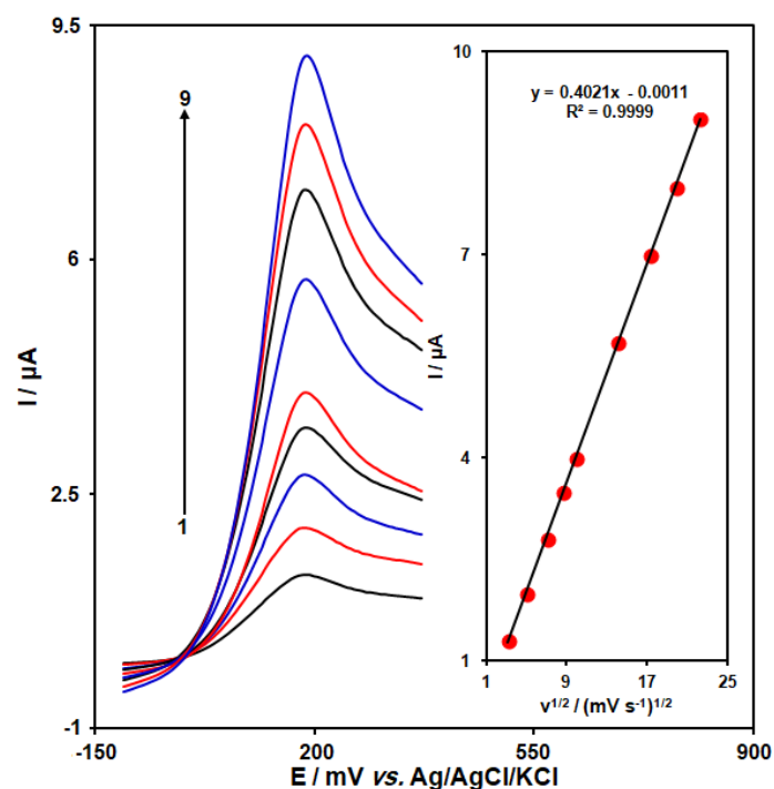
Fig. 2. LSV of Cu/SPE in 0.1 M PBS (pH 7.0) containing 200.0 \mu\text{M} norepinephrine at various scan rates; numbers 1-9 correspond to 10, 25, 50, 75, 100, 200, 300, 400 and 500 \text{mV s}^{-1} , respectively. Inset: variation of cathodic peak current vs. v^{1/2}
