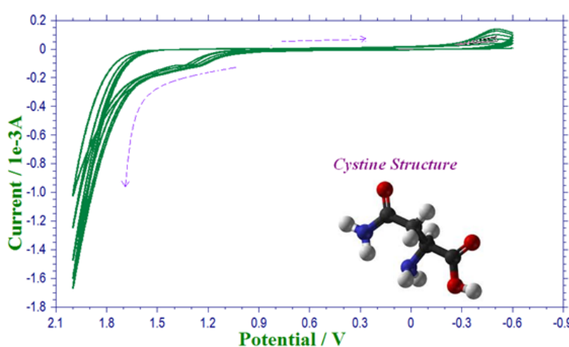
Fig. 1. Polymerization with L-Cystine at GCE (Scan rate 0.1 v/s and 0.1 m phosphate buffer solution of pH -7.0) inset structure of L-Cystine
