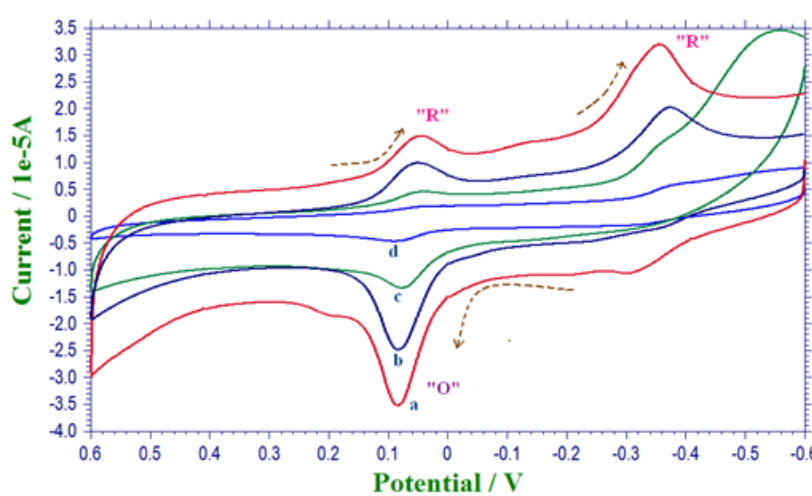
Fig. 4. Cyclic Voltammograms for the electrochemical response of DA at different electrodes in phosphate buffer solution of pH -7. a) bare GCE, b) MWCNTs/GCE, c) Poly(L-Cys)/GCE and d) MWCNTs/Poly(L-Cys)/GCE
