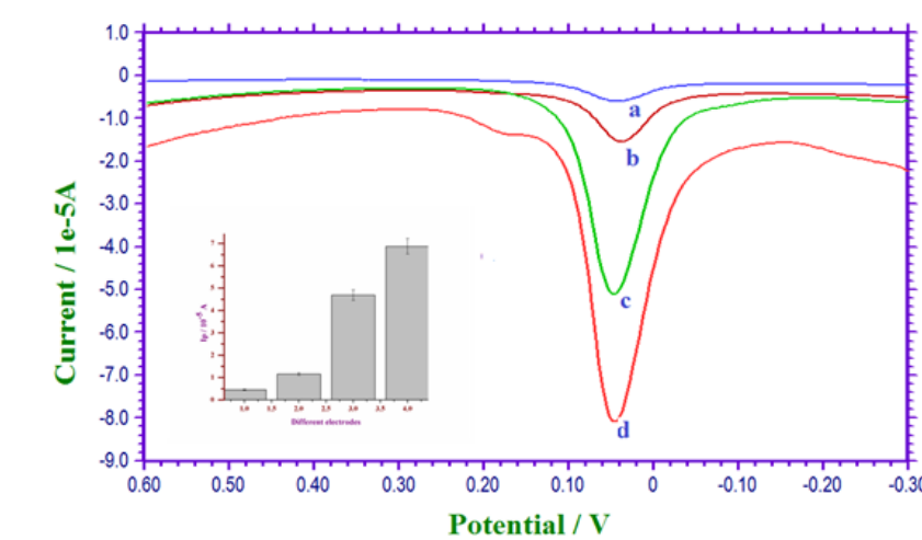
Fig. 3. Differential pulse voltammograms for the electrochemical response of 1 mM DA at a) bare/GCE b) MWCNTs/GCE c) Poly (L-Cys)/GCE d) MWCNTs/Poly(L-Cys)/GCE in a phosphate buffer solution of pH -7. Inset is the bar diagram illustrating different electrodes versus peak currents of 1 mM DA
