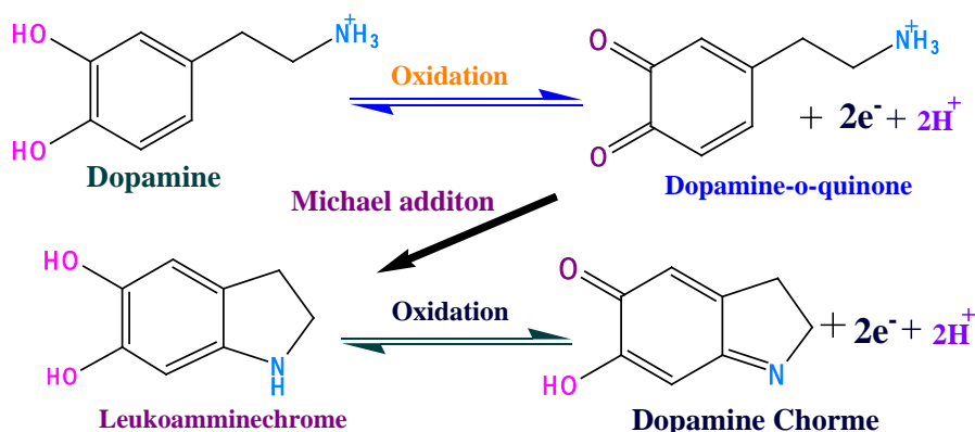
Scheme 1. Electrochemical redox mechanism of dopamine
