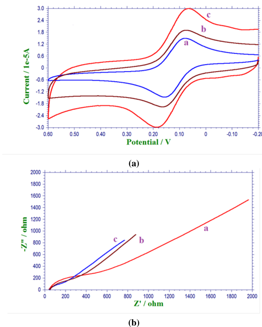
Fig. 2. (a) Cyclic Voltammograms of 1 mM [\text{Fe}(\text{CN})_6]^{-3/4} in 1 M KCl solution with a scan rate of 0.1\text{V s}^{-1} at a) bare/GCE b) Poly(L-Cys)/GCE c) MWCNTs/Poly(L-Cys)/GCE; (b) Nyquist plots for a) Bare/GCE b) Poly(L-Cys)/GCE c) MWCNTs/Poly(L-Cys)/GCE
