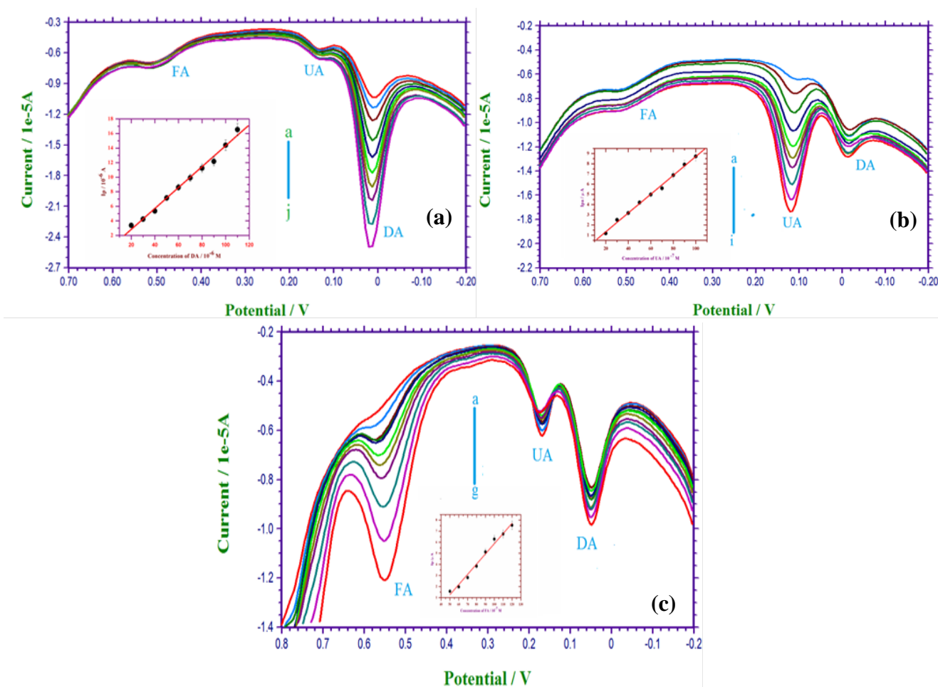
Fig. 8. (a) DPVs corresponding to the simultaneous determination of DA, in the presence of UA (100 μM) and FA (50 μM) with different concentrations of DA, i.e., 20 μM to 110 μM (a to j) at MWCNTs/poly (L-Cys)/GCE in PBS of pH 7.0; (b) DPVs corresponding to simultaneous determination of UA, in the presence of DA (30 μM) and FA (50 μM) with different concentrations of UA, i.e., 20 μM to 100 μM (a to i) at MWCNTs/poly (L-Cys)/GCE in PBS of pH 7.0; (c) DPVs corresponding to simultaneous determination of FA, in the presence of DA (30 μM) and UA (100 μM) with different concentrations of FA i.e., 30 μM to 130 μM (a to g) at a MWCNTs/poly (L-Cys)/GCE in PBS of pH 7.0
